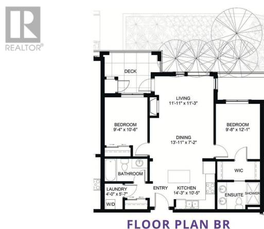
FLOOR PLAN BR
