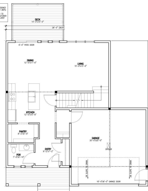
FIRST FLOOR PLAN SCALE: 3/16" = 1'-0"
